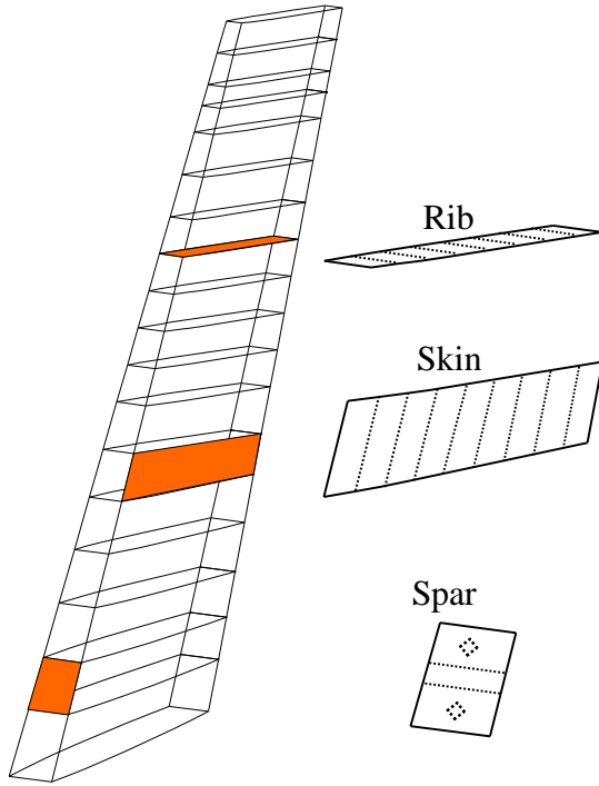
Fig. 2 VTP structure assembly of rib, skin, and spar panels
