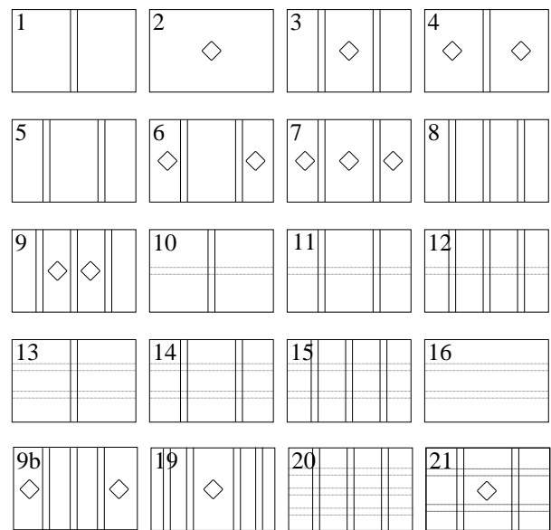
Fig. 5 Spar panel configurations that can be chosen in optimisation
