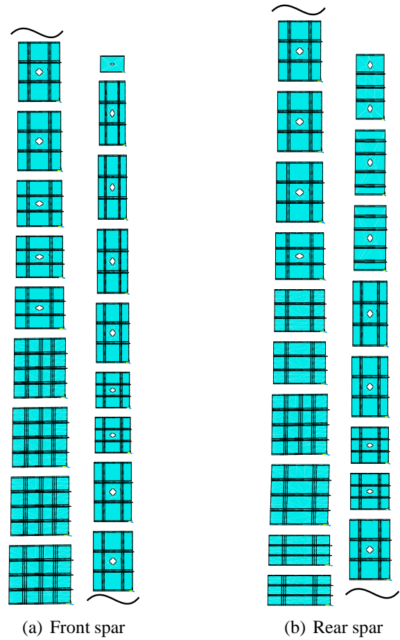
Fig. 6 Optimised designs (with realistic load-cases)
