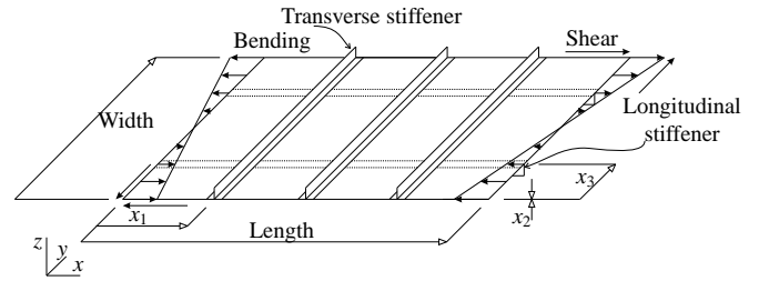
Fig. 3 Parameterised panel
