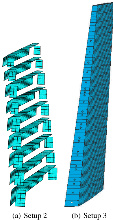
Fig. 7 Optimised designs (loadcases are not realistic)
